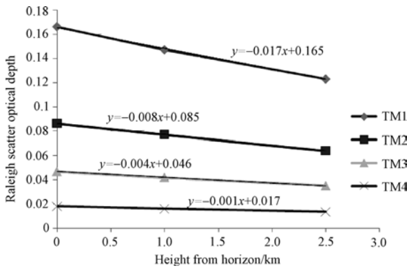
Fig. 3 Rayleigh scatter optical depth
